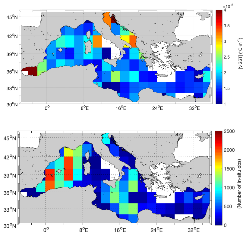
Figure 11. Top panel: |\nabla SST| binned in 1^\circ \times 1^\circ boxes, computed along the positions occupied by the drifting buoys during the period 2012–2016. Bottom panel: Number of in-situ surface-currents observations laying in each of the 1^\circ \times 1^\circ boxes.
